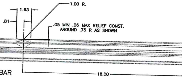
DETAIL OF HEAD 2 X SIZE
