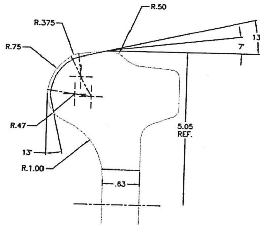
DETAIL OF HEAD 2 X SIZE
